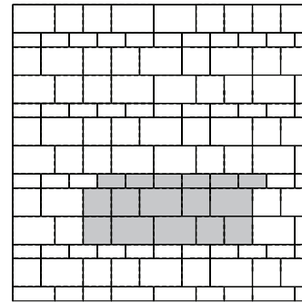
Pattern C (Running Bond with Random Bundle)
